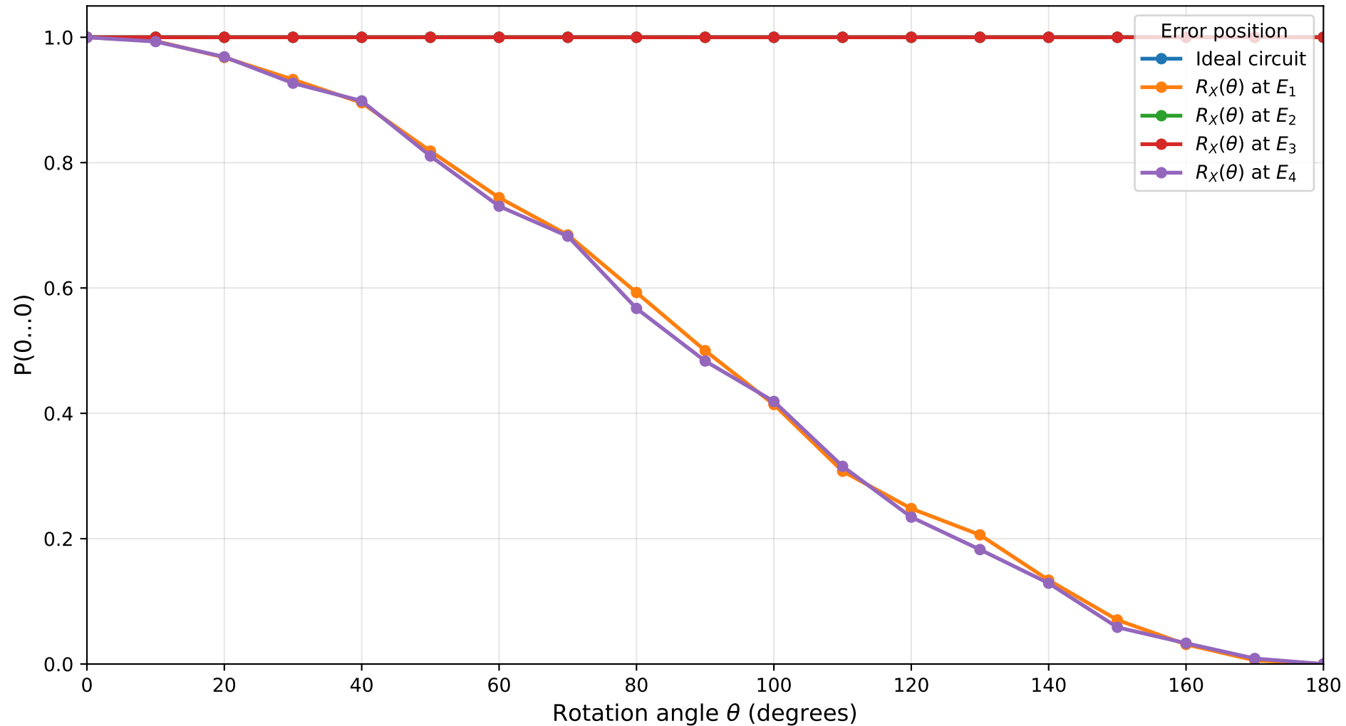
Probability under X-Axis Rotation Errors Constant 0, n=7 , target qubit=4, shots=1024
