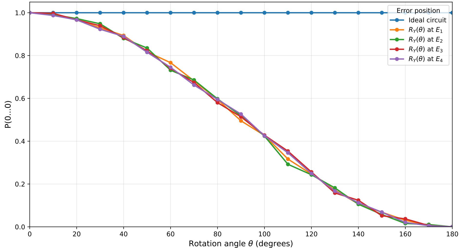
Probability under Y-Axis Rotation Errors Constant 0, n=7 , target qubit=4, shots=1024
