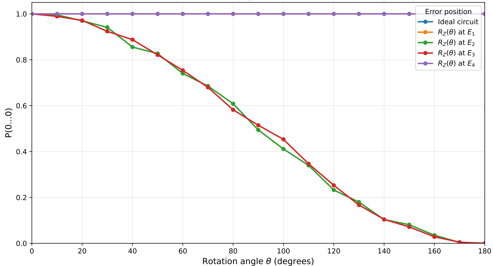
Probability under Z-Axis Rotation Errors Constant 0, n=7 , target qubit=4, shots=1024
