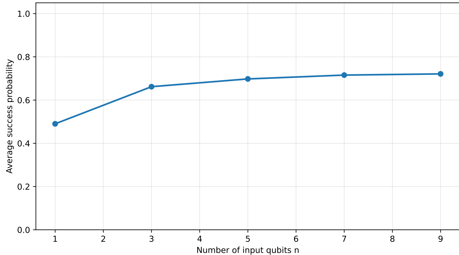
Scalability under \mathcal{E}_4 after final H noise axis=X, \theta=90^\circ , shots=1024
