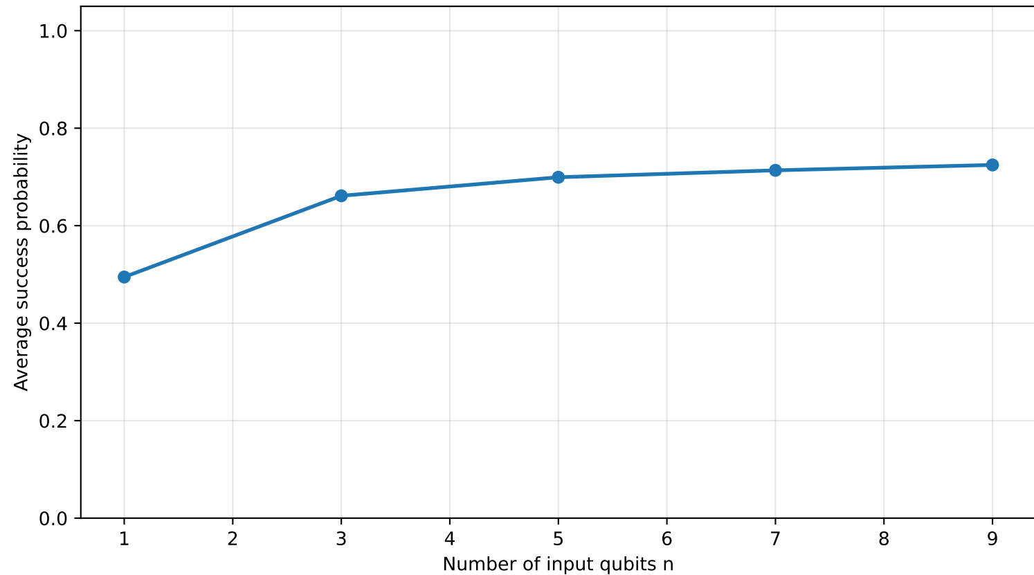
Scalability under \mathcal{E}_4 after final H noise axis=Y, \theta=90^\circ , shots=1024
