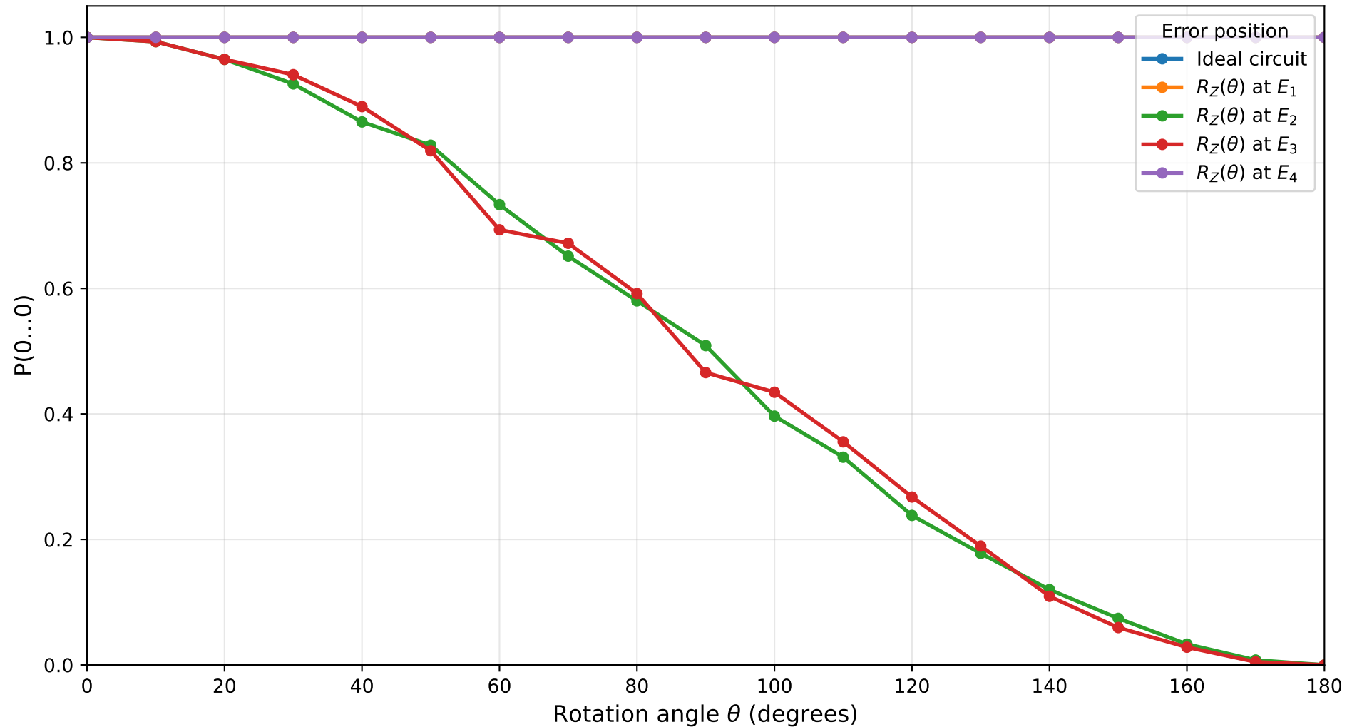
Probability under Z-Axis Rotation Errors Constant 1, n=9 , target qubit=4, shots=1024
