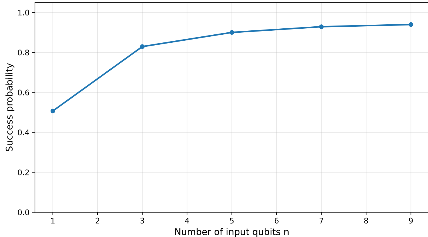
Scalability for balanced under R_Y(\theta) at E_3 noise axis=Y, \theta=90^\circ , shots=1024
