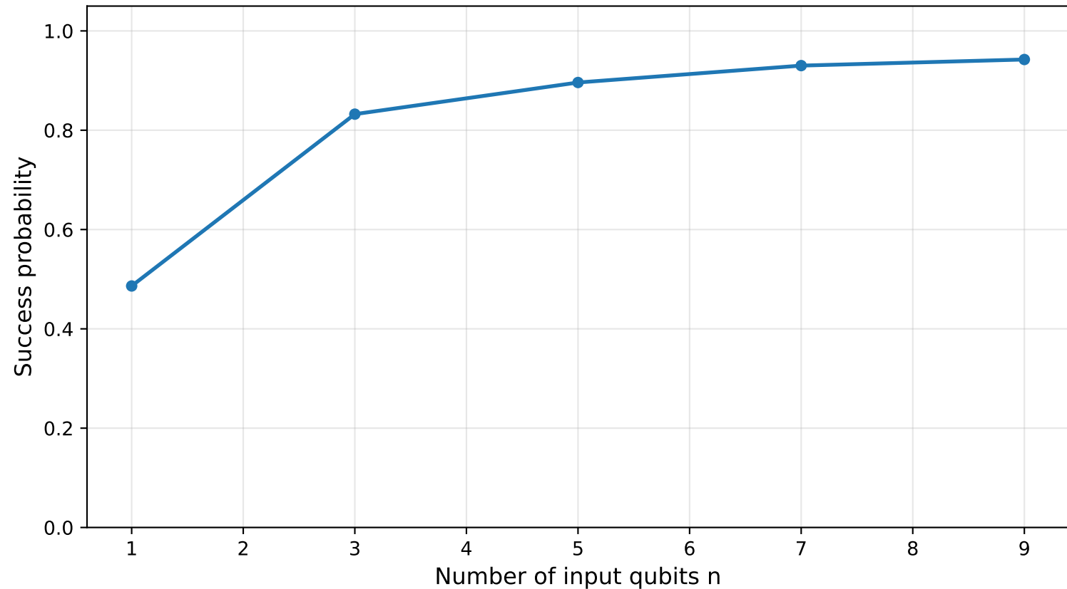
Scalability for balanced under R_Z(\theta) at E_3 noise axis=Z, \theta=90^\circ , shots=1024
