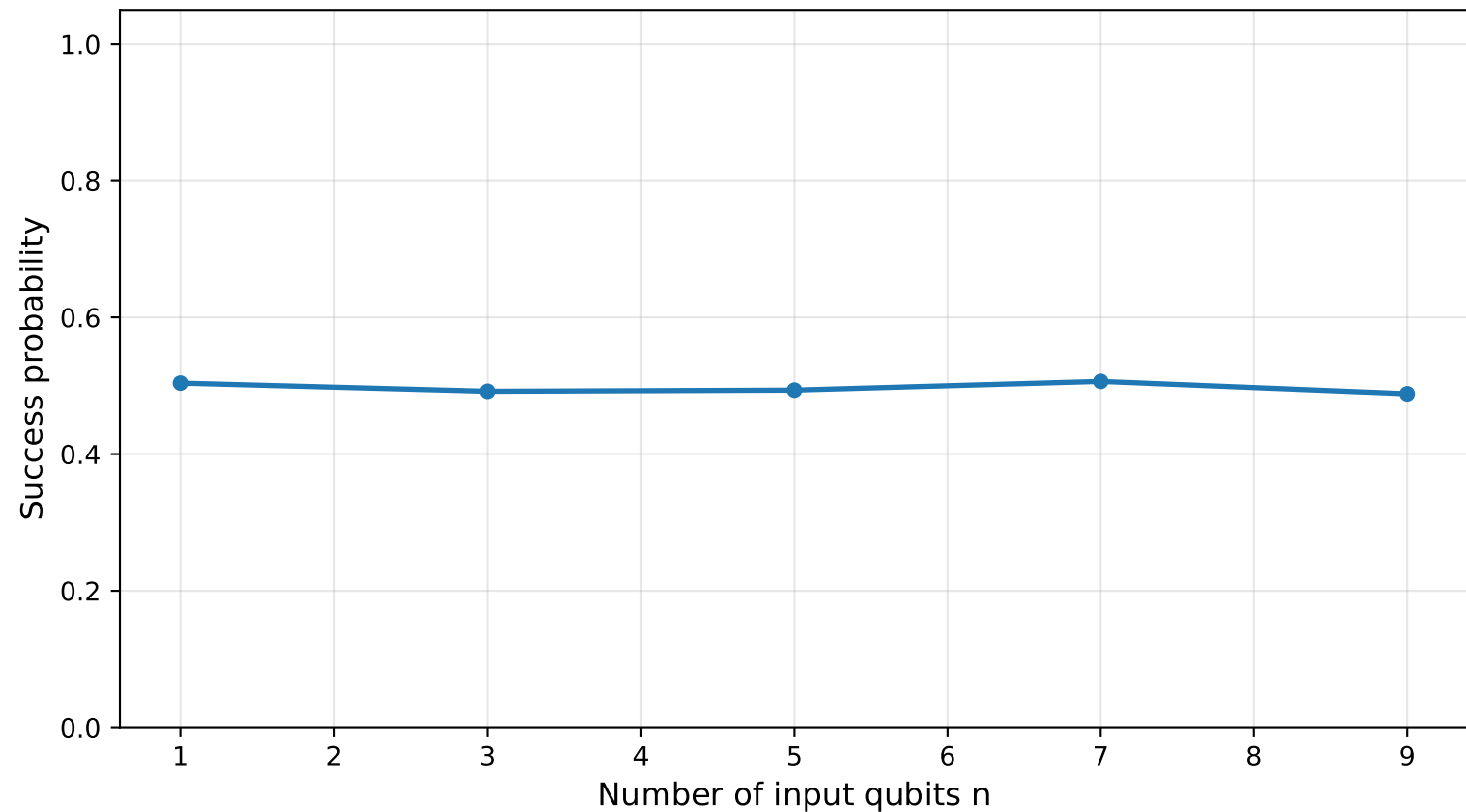
Scalability for constant_0 under R_Y(\theta) at E_3 noise axis=Y, \theta=90^\circ , shots=1024
