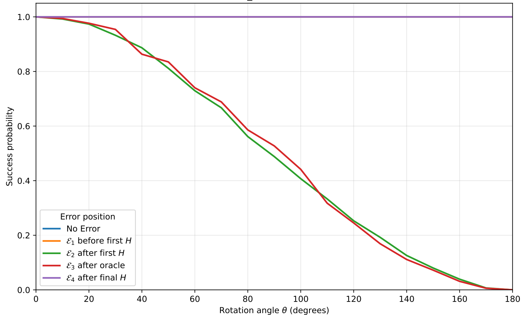
success under rotation errors function=constant_1, n=9, axis=Z, shots=1024
