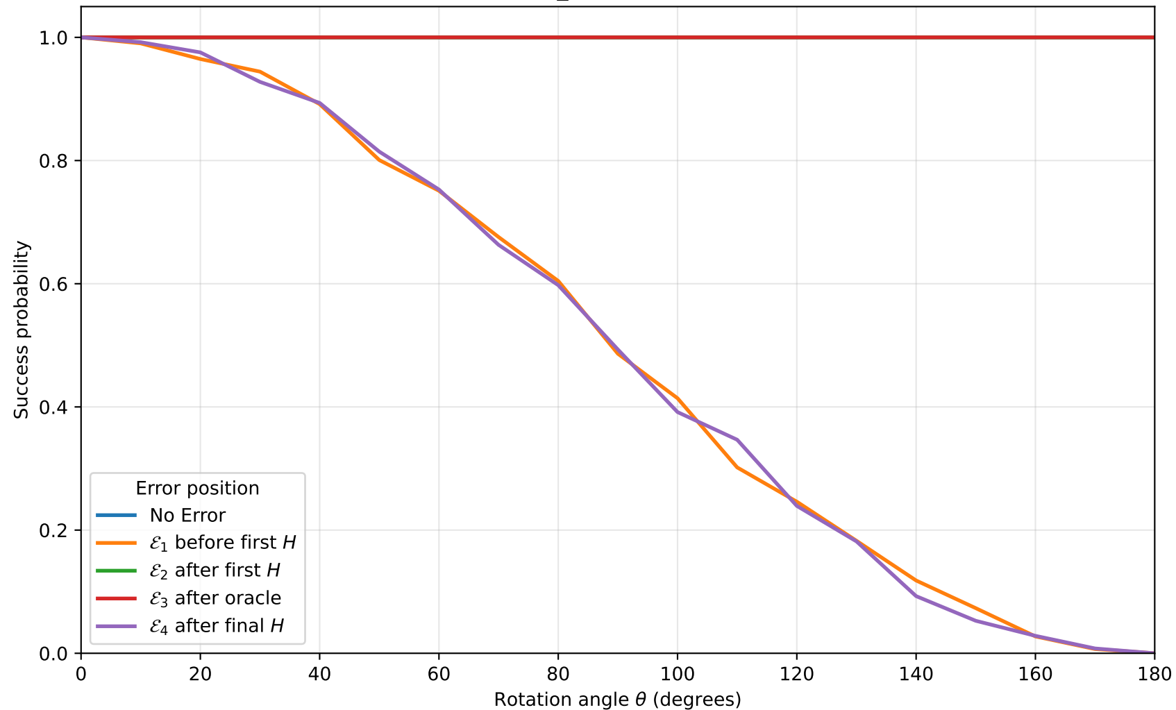
success under rotation errors function=constant_0, n=9, axis=X, shots=1024
