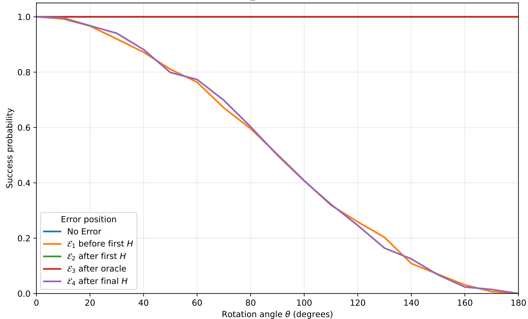
success under rotation errors function=constant_1, n=9, axis=X, shots=1024
