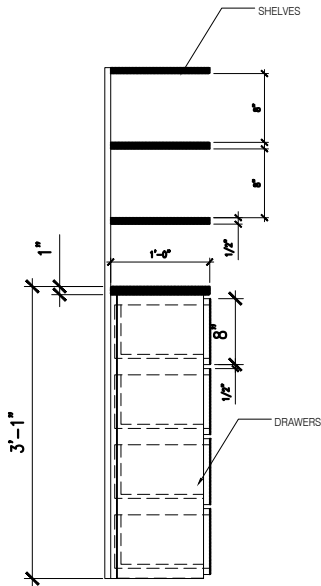
SECTION VIEW (A)
