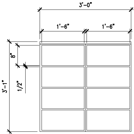
BASE CABINET VIEW
