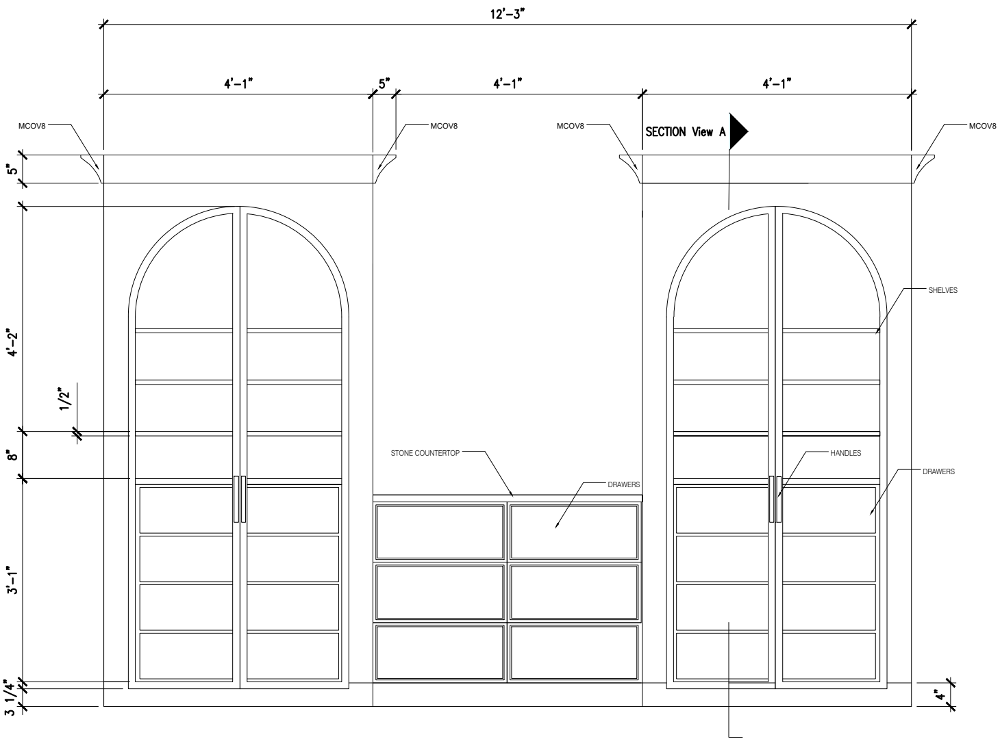
FRONT VIEW
