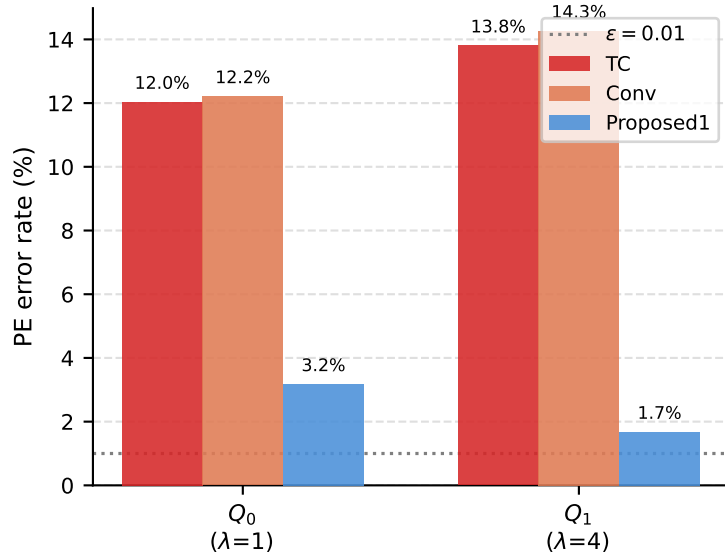
(b) Per-plane 2-bit PE error rate
