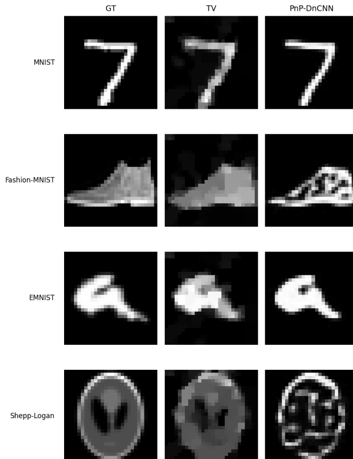
Figure 7: Qualitative reconstructions under distribution shift. The learned prior recovers structure well on MNIST and EMNIST (both stroke-like), but imposes hallucinated digit/stroke-like structure on Fashion-MNIST and the CT phantom, both structurally unlike the training distribution.
