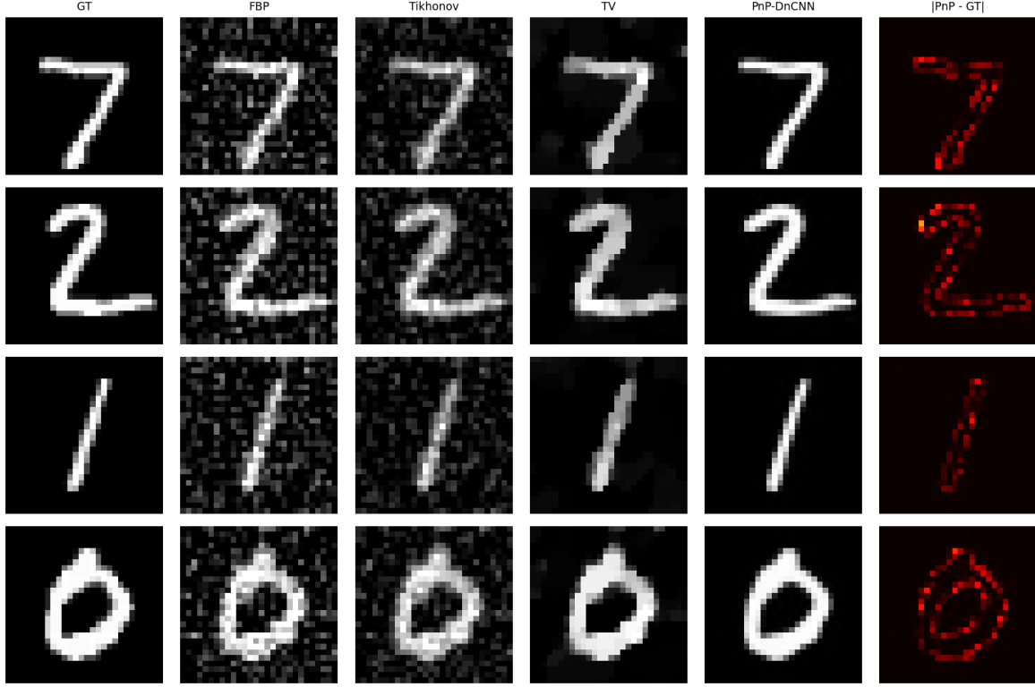
Figure 3: Qualitative in-distribution reconstructions at \sigma = 0.05 , 20 angles. Each row is one test digit; columns show the ground truth, the three classical baselines, PnP-DnCNN, and the absolute error map |\hat{x}_{\text{PnP}} - x| (brighter = larger error). FBP and Tikhonov retain visible measurement noise; TV produces flat, blocky regions; PnP-DnCNN recovers the sharpest, most faithful strokes. The error maps show that residual error is concentrated almost entirely along stroke boundaries, with near-zero error in flat background and interior regions.
