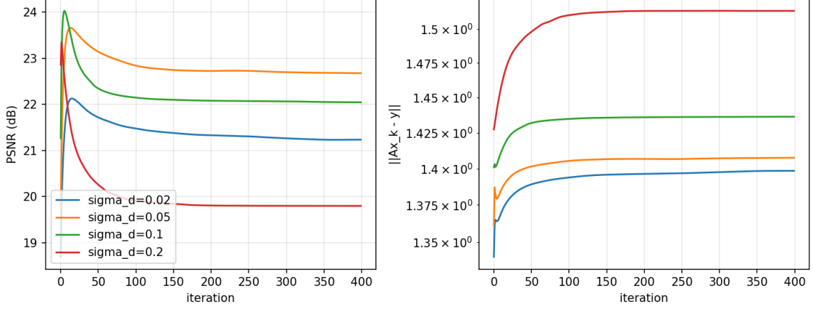
Figure 4: PnP-PGD convergence behavior for several denoising strengths \sigma_d (50 test images, \sigma = 0.05 , 20 angles). Left: PSNR vs. iteration, peaking early then decaying. Right: data-fidelity residual vs. iteration, rising and plateauing rather than decreasing.
