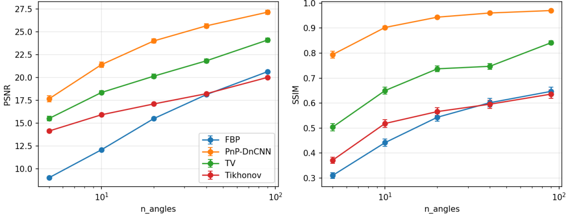
Figure 2: Reconstruction accuracy (PSNR, left; SSIM, right) vs. number of projection angles, for all four methods at a fixed measurement noise \sigma = 0.05 . PnP-DnCNN is the top performer across the full range tested (5 to 90 angles), with its largest relative advantage at the fewest angles. Error bars denote 95% confidence intervals over 200 test images.
