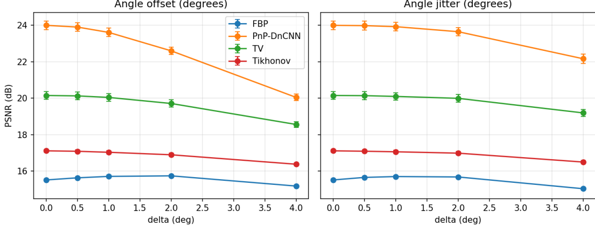
Figure 5: Test PSNR under forward-model mismatch, as a function of angular error \delta (degrees), for a constant angle offset (left) and independent per-angle jitter (right). All hyperparameters are frozen at their nominal ( \delta = 0 ) values and not retuned per mismatch level. PnP-DnCNN remains the most accurate method throughout the tested range, but degrades faster than TV, particularly under the systematic offset: its advantage over TV narrows from +3.85 dB at \delta = 0 to +1.48 dB at \delta = 4^\circ . Error bars denote 95% confidence intervals over 200 test images.
