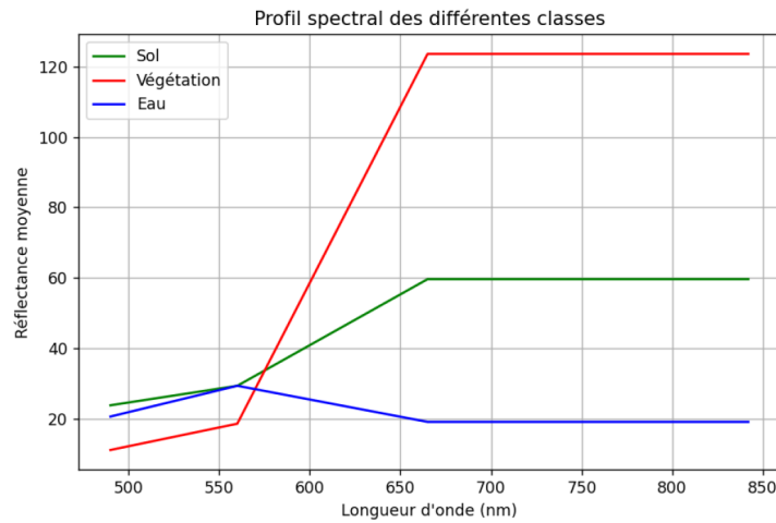
Figure 9: Mean spectral signatures (reflectance vs. wavelength) for the soil, vegetation, and water ROIs.
