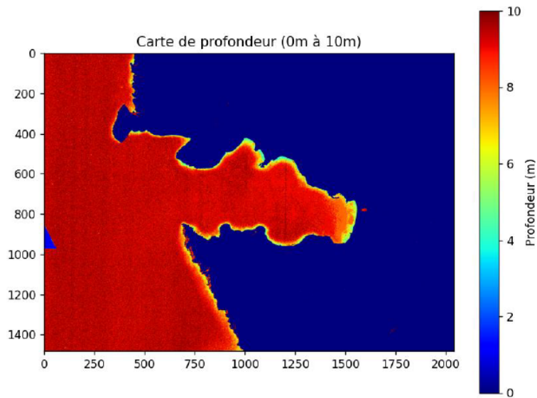
Figure 5: Final estimated depth map (0–10 m), obtained via affine calibration of the corrected bathymetric index.
