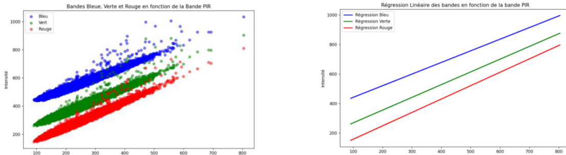
Figure 2: Left: blue, green, and red band reflectance as a function of the NIR band over the offshore reference area. Right: fitted linear regressions used for surface-reflection correction.
