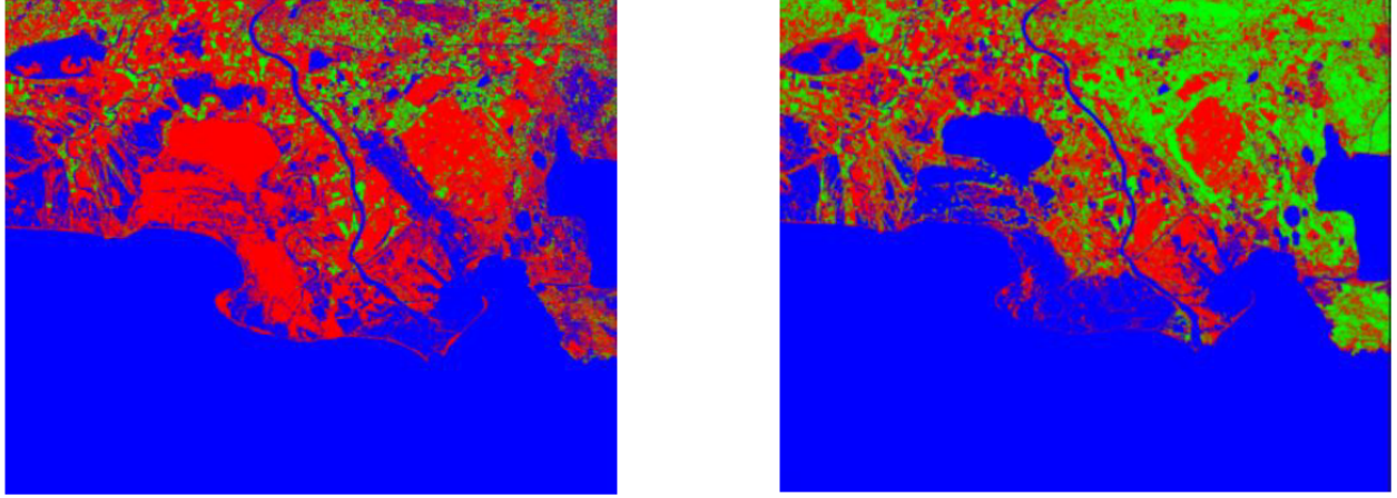
Figure 10: Classification of the Camargue scene using Euclidean distance (left) and the Spectral Angle Mapper (right).
