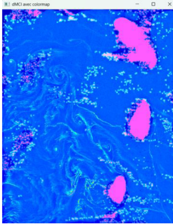
Figure 13: Differential chlorophyll index (dMCI), with land/cloud mask overlaid, highlighting local anomalies attributed to floating algae.
