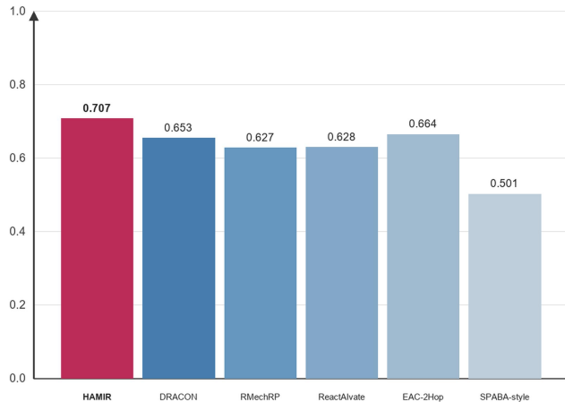
USPTO-FULL
