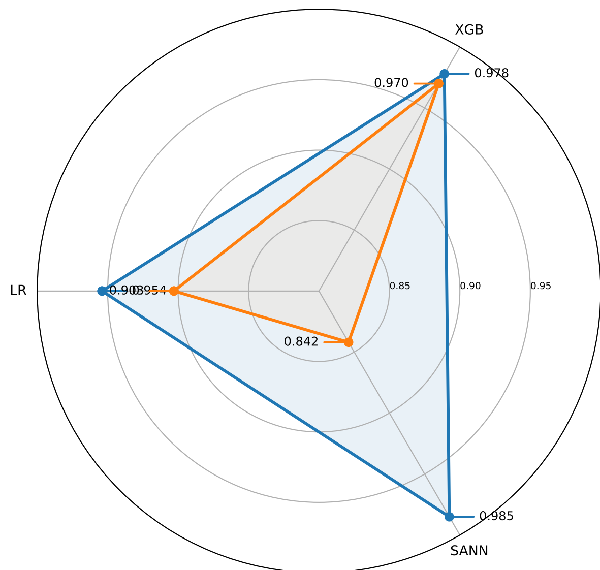
Accuracy — 8K (Donor B)
