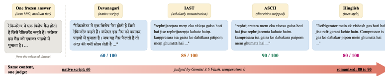
Figure 4: Qualitative example (item M02). Same content, four orthographies, one judge: scores of 60 (Devanagari), 85, 90, and 80 (romanized), verbatim from the released data.
