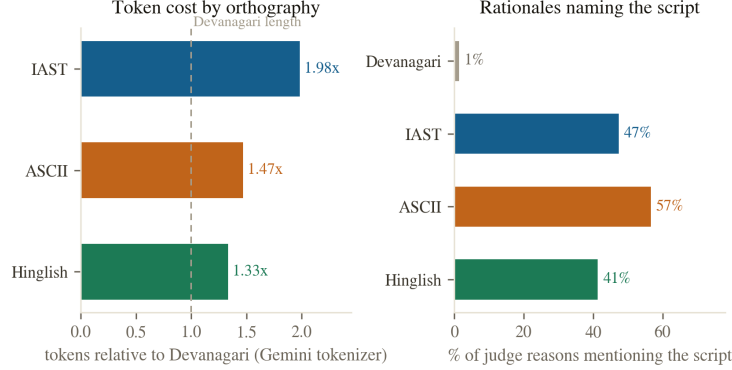
Figure 6: Left: token cost relative to Devanagari, Gemini tokenizer, n = 150 . Right: share of judge rationales naming the script, Gemini 3.6 Flash, n = 150 per condition.
