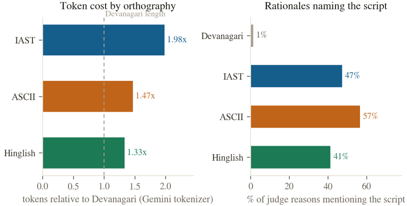
Figure 7: Left: token cost relative to Devanagari, Gemini tokenizer, n = 150 . Right: share of judge rationales naming the script, Gemini 3.6 Flash, n = 150 per condition.
