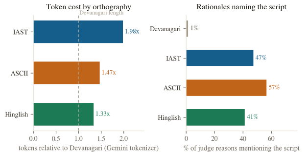
Figure 6: Left: the same content costs 1.33 to 1.98 times as many tokens romanized as in Devanagari under the Gemini tokenizer (mean over 150 items; Devanagari mean 93 tokens). Right: share of the judge’s one-sentence rationales that mention script, romanization, or transliteration, by condition, under Gemini 3.6 Flash ( n = 150 per condition). The judge names the script on 41 to 57 percent of romanized items and on 1 percent of Devanagari items.
