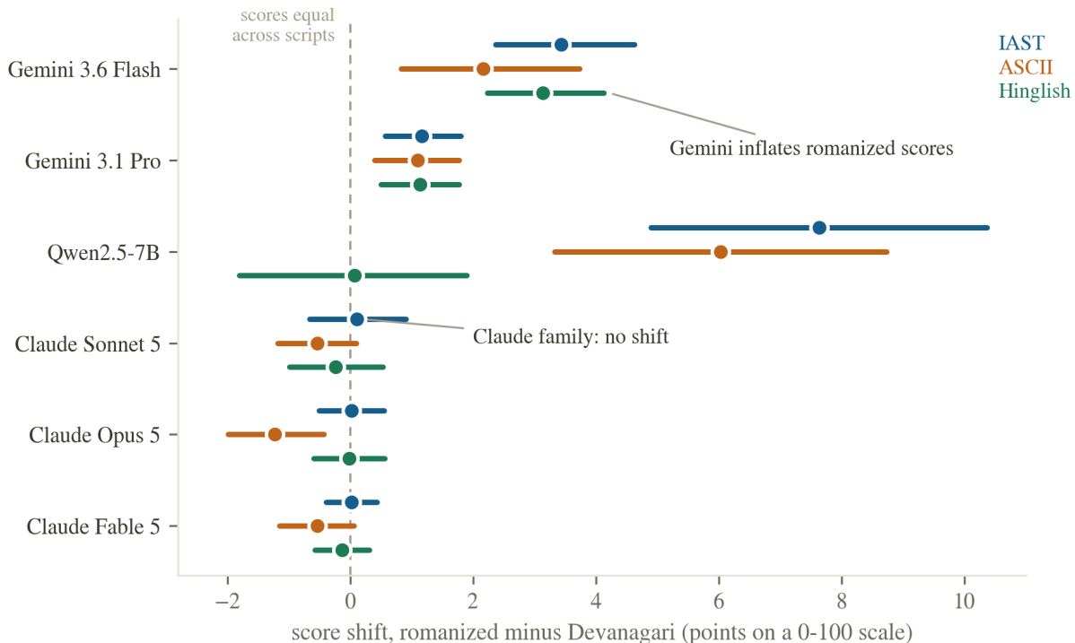
Figure 3: Score shift by judge and romanization, with 95 percent bootstrap confidence intervals. Each row group is one judge; each interval is the mean within-item shift (romanized minus Devanagari) over n = 150 paired items. Read intervals against the dashed zero line: right of zero means romanized content scored higher than the same content in Devanagari. Both Gemini judges and Qwen (on formal romanizations) sit right of zero; all three Claude judges straddle zero except Opus 5 on ASCII.
