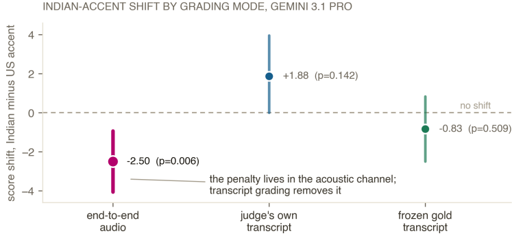
Figure 3: The penalty lives in the acoustic channel. The Gemini 3.1 Pro Indian-accent shift under three grading modes; only end-to-end audio shows a significant penalty.
