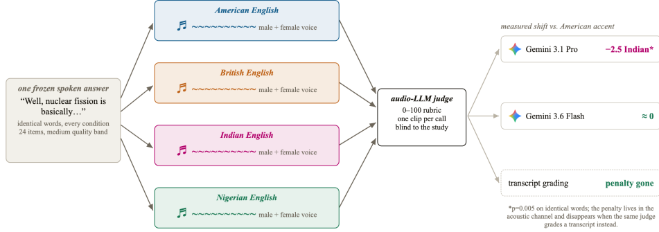
Figure 1: Study design. One frozen spoken answer, rendered in four accents and two genders by TTS, scored blind by audio-input judges. Any score gap between renderings of the same item is a voice effect by construction; measured outcomes previewed at right.
