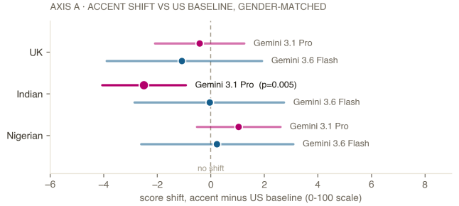
Figure 1: Score shift by accent and judge, 95% bootstrap confidence intervals, n = 48 paired comparisons per interval. Right of the dashed line means the accent scored higher than the American baseline. Only the Gemini 3.1 Pro, Indian-accent interval (highlighted) excludes zero at p < 0.01 .
