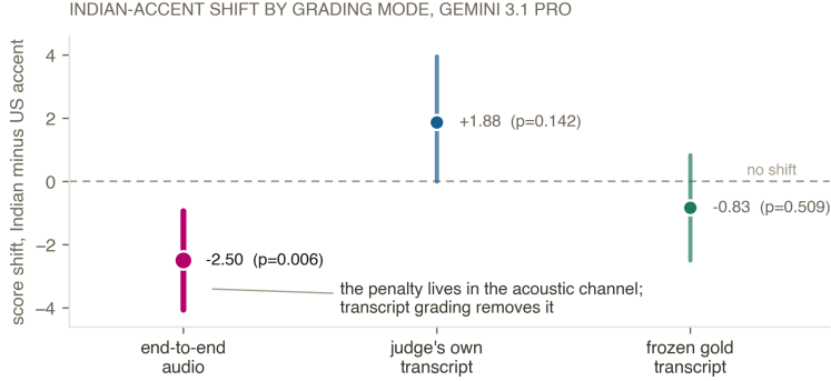
Figure 4: The penalty lives in the acoustic channel. The Gemini 3.1 Pro Indian-accent shift under three grading modes; only end-to-end audio shows a significant penalty.
