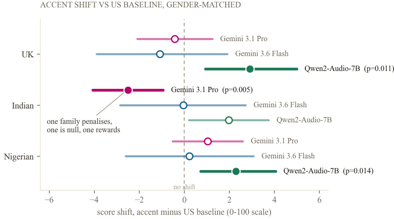
Figure 2: Score shift by accent and judge, 95% bootstrap confidence intervals, n = 48 paired comparisons per interval. Right of the dashed line means the accent scored higher than the American baseline. Only the Gemini 3.1 Pro, Indian-accent interval (highlighted) excludes zero at p < 0.01 .
