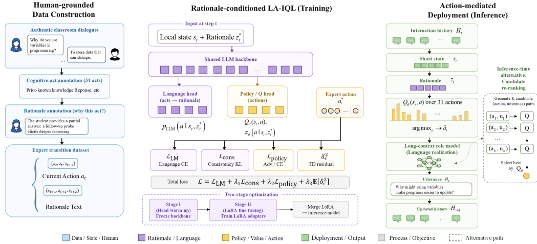
Fig. 3. LA-IQL framework and technical flow. Human-grounded classroom dialogue and cognitive-act annotations are converted into rationale-augmented expert transitions (left). Rationale-conditioned LA-IQL jointly trains language and policy/value components with language, consistency, policy, and temporal-difference objectives (center). At inference, the learned policy selects an interaction action and a long-context role model realizes it as an utterance; candidate re-ranking is shown as an inference-time alternative (right).
