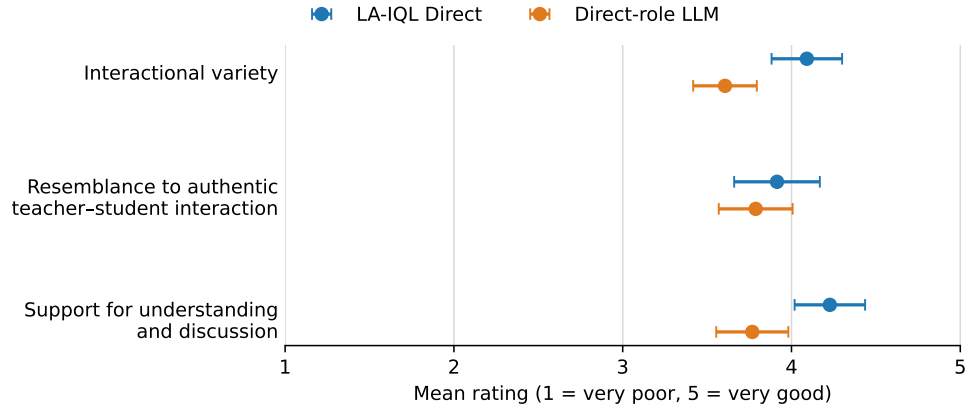
Fig. 4. Supplementary excerpt-level human evaluation. Points are means of participant-level ratings across six excerpts per system and dimension; error bars are 95% confidence intervals. The figure contains only the main LA-IQL Direct system and the Direct-role LLM generation baseline. The first and third dimensions differ under Holm-corrected paired tests ( p < .001 ), whereas perceived resemblance does not ( p = .299 ).
