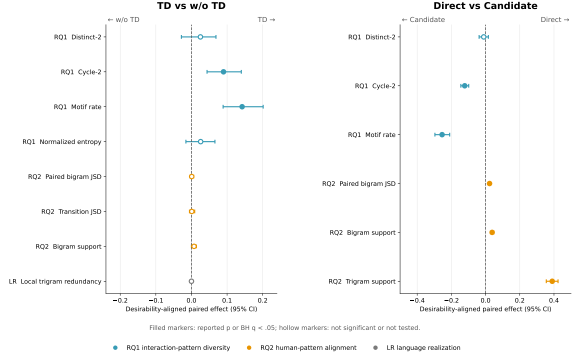
Fig. 5. Desirability-aligned paired effects for the fixed-checkpoint TD contrast and Direct-Candidate system contrast. For metrics marked ↓ in the result tables, the reported difference and interval are multiplied by -1 so that positive values consistently favor the first named system (TD or Direct). Horizontal bars are percentile 95% intervals from 10,000 paired bootstrap resamples clustered by the 10 held-out lessons. Filled markers denote a reported p < .05 or BH-adjusted q < .05 ; hollow markers denote a non-significant or untested comparison. The Direct-Candidate panel is a descriptive system-level comparison because rationale temperature also differs between configurations. LR marks the auxiliary language-realization diagnostic rather than an evaluation goal.
