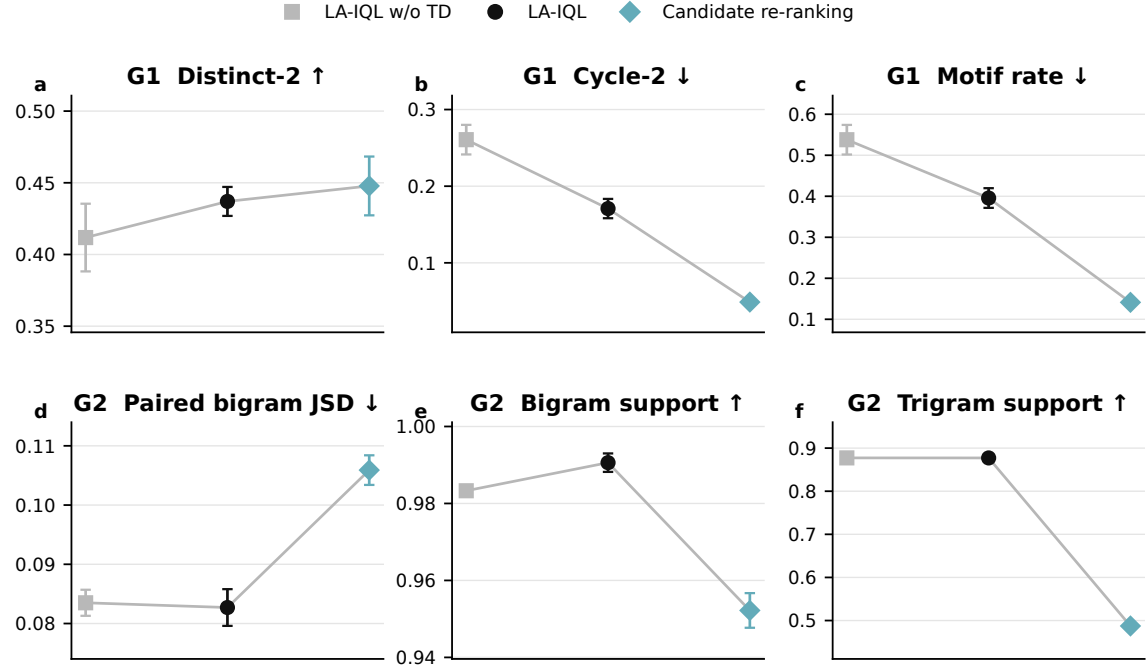
Fig. 5. Core G1 and G2 results for the three learned-system configurations. Points show means and error bars show population standard deviations across seeds 42–44, with 10 held-out lessons per seed. Connecting lines are visual guides rather than temporal trajectories; arrows indicate the desirable metric direction.
