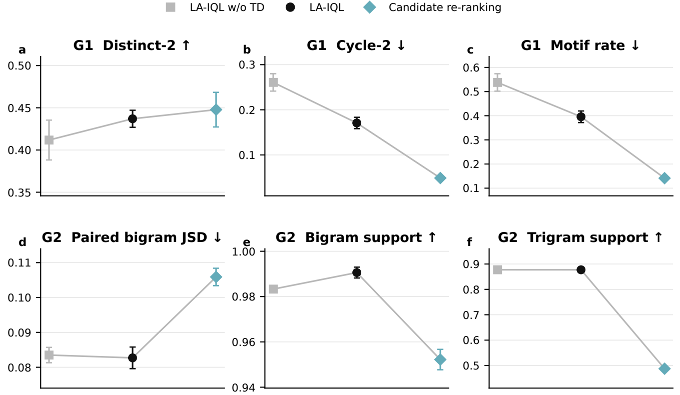
Figure 5: Core G1 and G2 results for the three learned-system configurations. Points show means and error bars show population standard deviations across seeds 42–44, with 10 held-out lessons per seed. Connecting lines are visual guides rather than temporal trajectories; arrows indicate the desirable metric direction.
