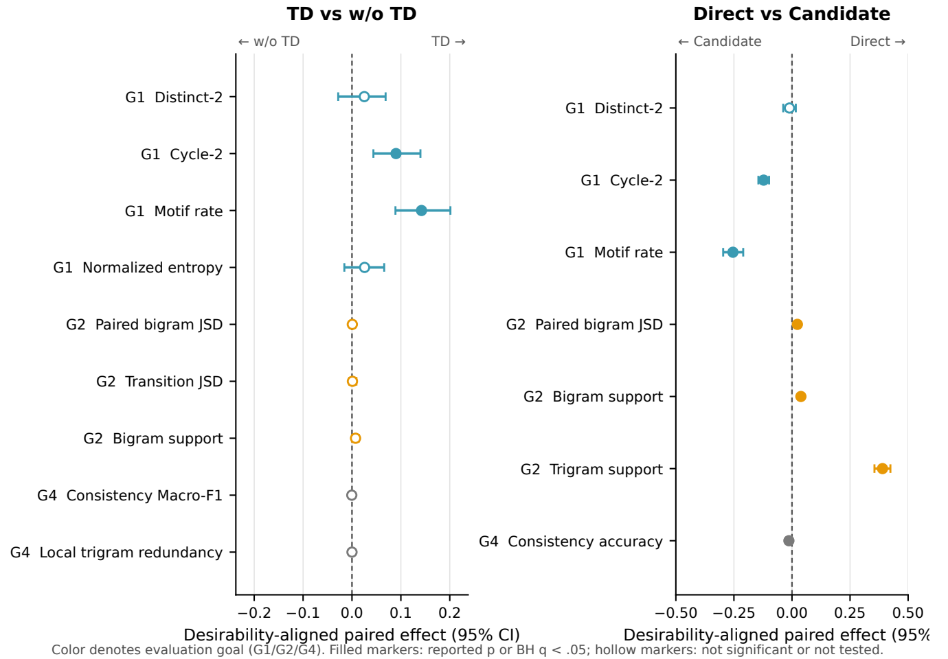
Figure 4: Desirability-aligned paired effects for temporal-difference training and decoding configuration. For metrics marked ↓ in the result tables, the reported difference and interval are multiplied by −1 so that positive values consistently favor the first named system (TD or Direct). Horizontal bars are percentile 95% intervals from 10,000 paired bootstrap resamples clustered by the 10 held-out lessons. Filled markers denote a reported p < .05 or BH-adjusted q < .05 ; hollow markers denote a non-significant or untested comparison. The Direct–Candidate panel is a descriptive system-level comparison because rationale temperature also differs between configurations.
