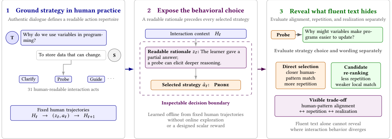
Figure 1: From human practice to inspectable language-mediated behavior. Authentic dialogue grounds trajectories over readable interaction acts; LA-IQL exposes a rationale and selected strategy before language realization; and the resulting action boundary supports separate evaluation of behavioral choice and surface expression. In our classroom testbed, this boundary reveals a trade-off: direct selection more closely matches held-out human action patterns, whereas candidate re-ranking reduces repetition but moves farther from those patterns.
