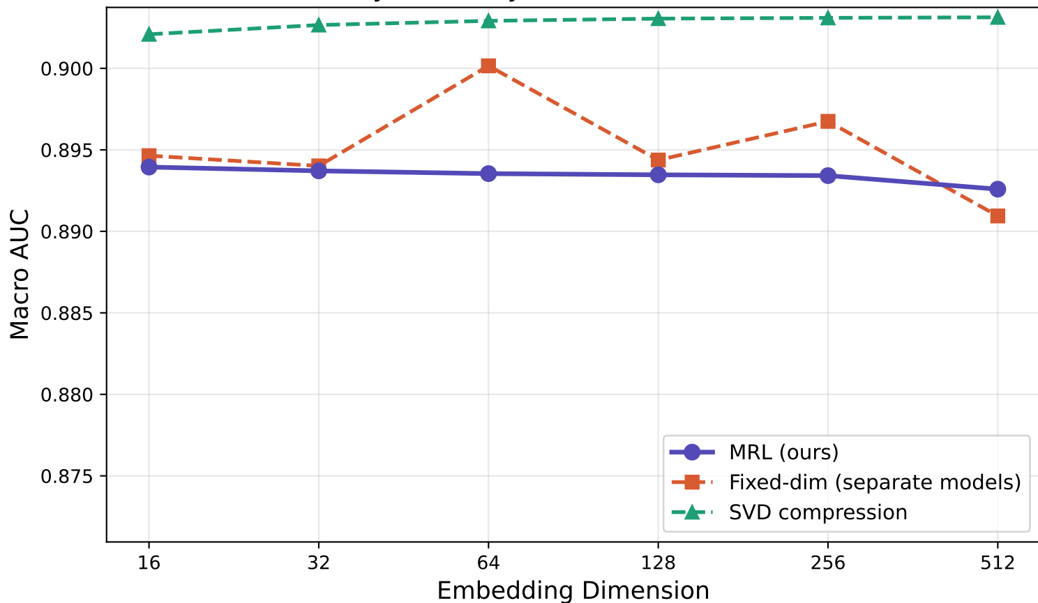
Accuracy-Efficiency Tradeoff: MRL vs Baselines
