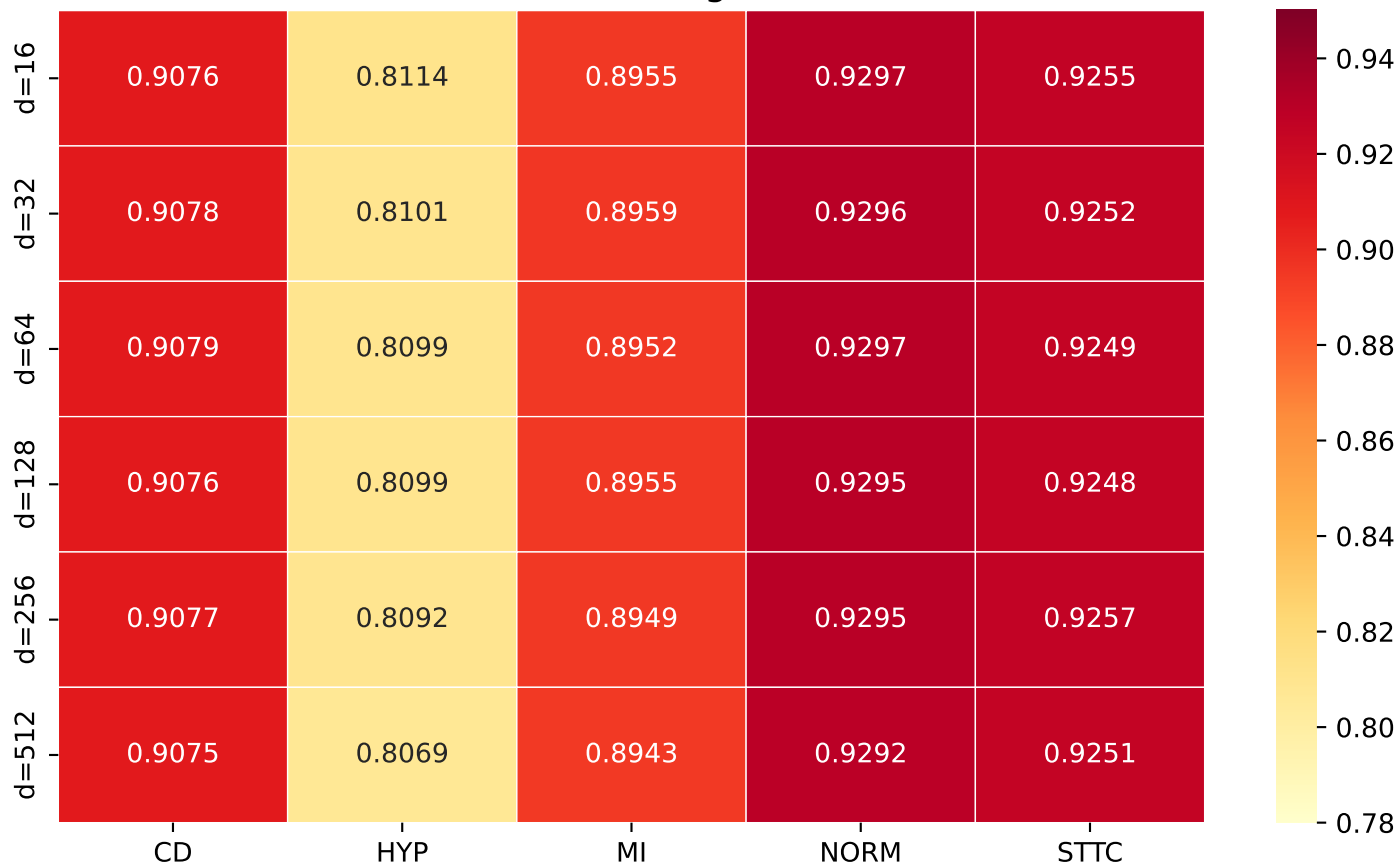
Per-class AUC Across Nesting Dimensions (MRL)
