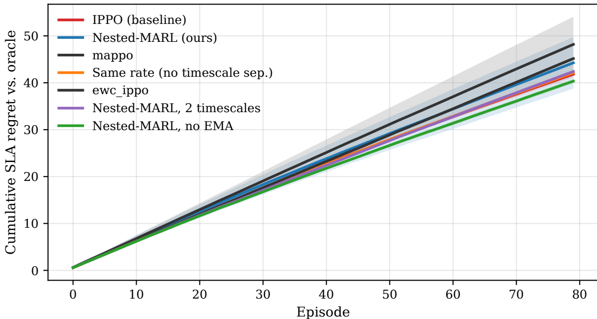
Cumulative regret under multi-timescale non-stationarity
