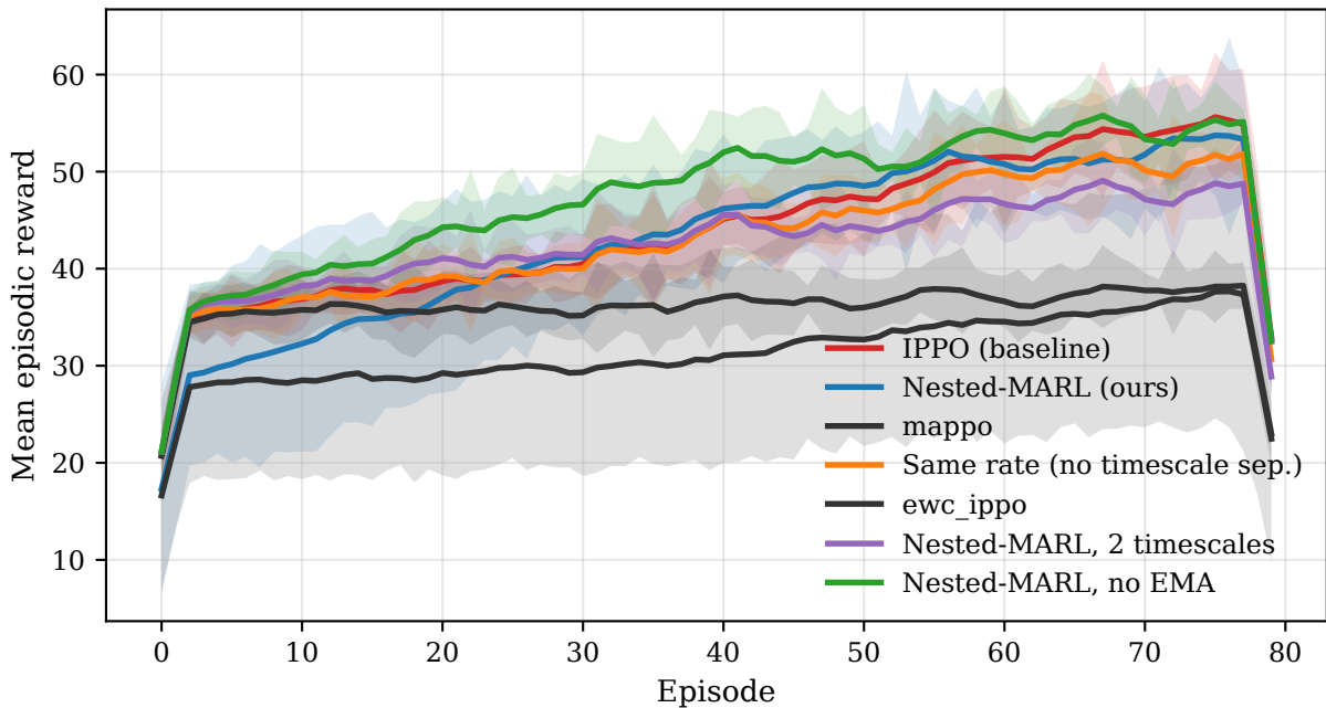
Learning curves under multi-timescale drift
