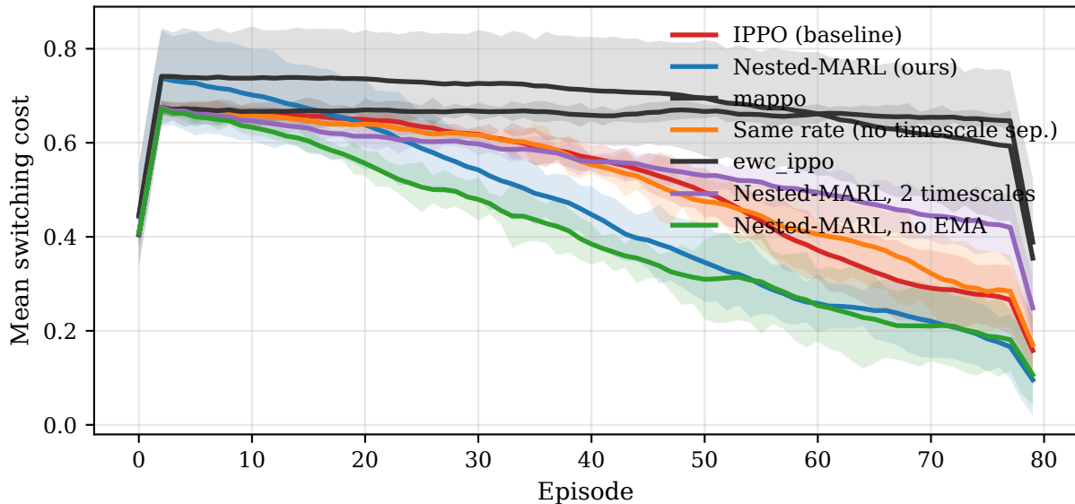
Policy stability: switching cost over training
