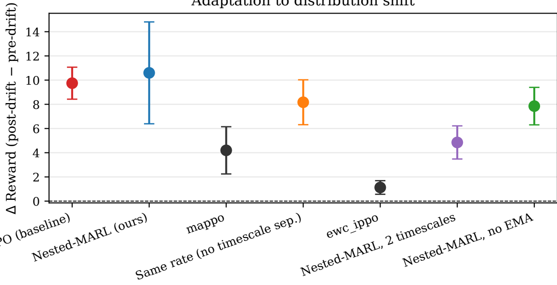
Adaptation to distribution shift
