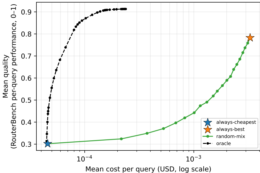
Routing headroom on RouterBench (static references)
