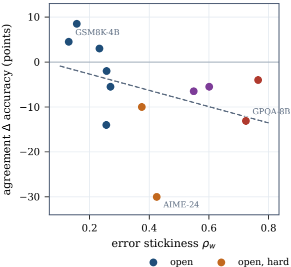
(a) Sticky errors predict collapse
