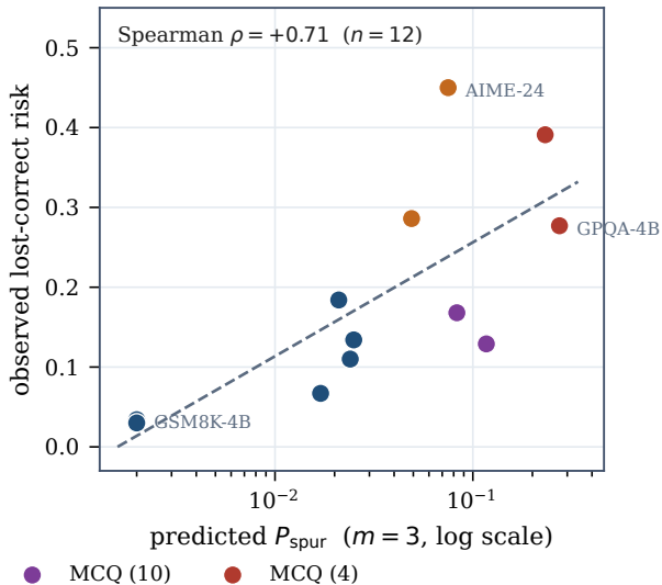
(b) Prediction tracks measurement
