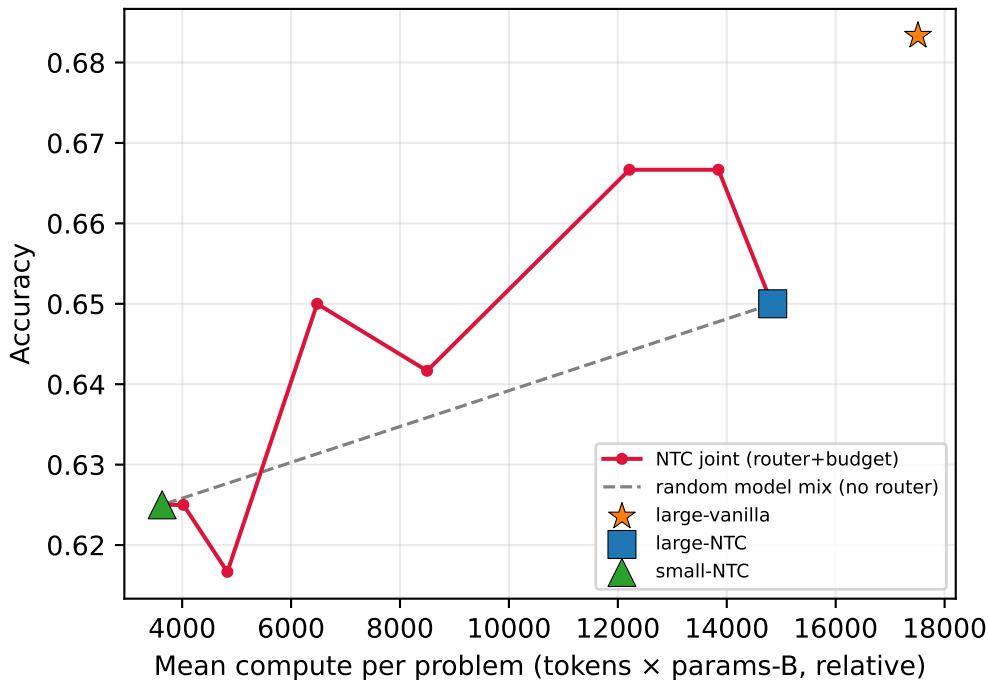
Joint model-routing + budget control · math500
