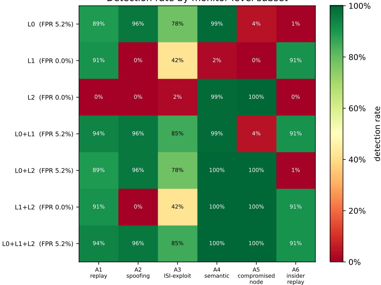
Detection rate by monitor level subset
