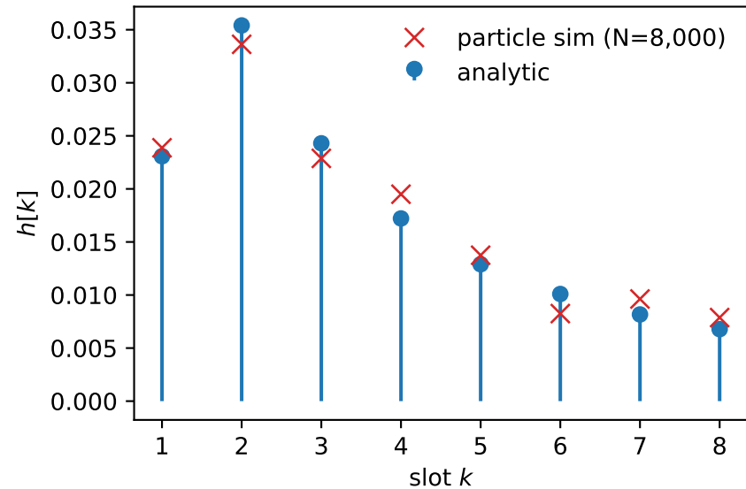
Discrete channel impulse response
