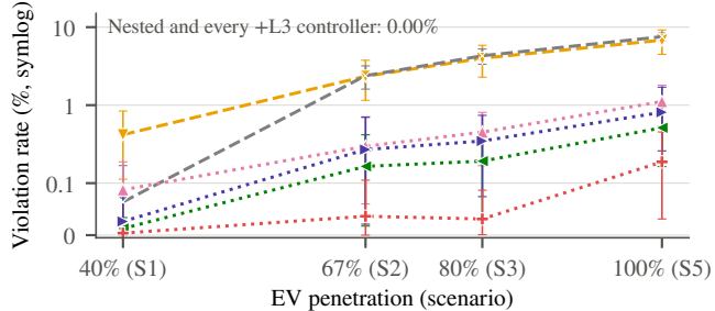
(b) Violation rate of controllers without Level 3
