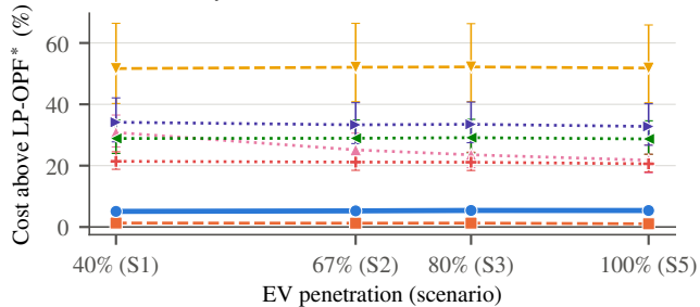
(a) Mean daily cost relative to LP-OPF* +L3
