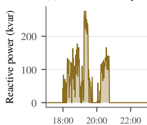
(c) Level-3 reactive power
