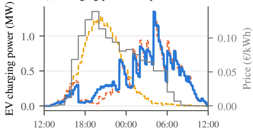
(a) Charging power and price
