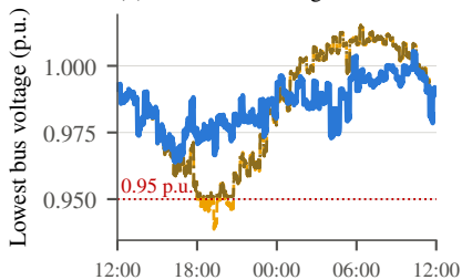
(b) Lowest bus voltage
