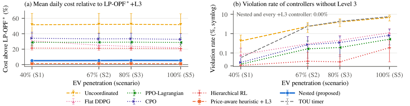
Fig. 5. (a) Mean daily energy cost relative to that of the perfect-foresight LP-OPF with Level 3 (ratio of means over the test days; 95% intervals from a bootstrap over days that keeps both methods' costs of a day together), and (b) violation rate of the controllers without Level 3 (symmetric-log axis), across S1, S2, S3 and S5. The nested controller and every “+L3” controller have no violations in these scenarios.
