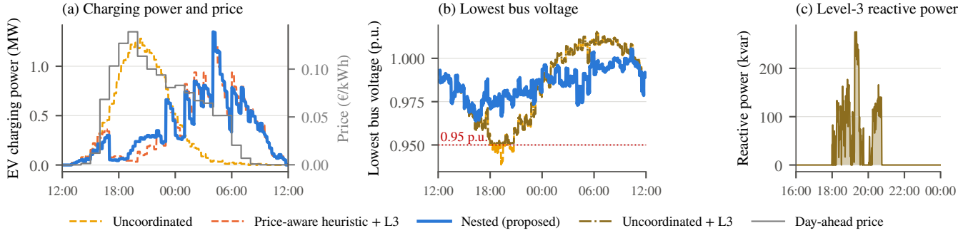
Fig. 4. Operation on a representative S3 test day (29 June 2024, the day with the median cost of uncoordinated charging; nested controller of training seed 0) at 60-s resolution. (a) Aggregate EV charging power and day-ahead price, (b) lowest bus voltage (uncoordinated charging with and without Level 3 coincide except where Level 3 acts), and (c) reactive power injected by Level 3 under uncoordinated charging; the heuristic and the nested controller need none on this day.
