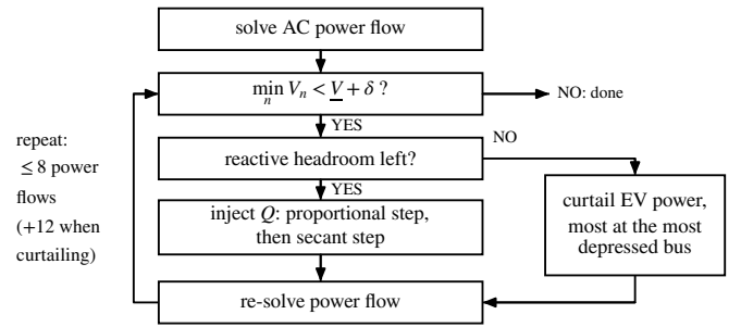
Fig. 3. Level-3 correction inside one 60-s step.
