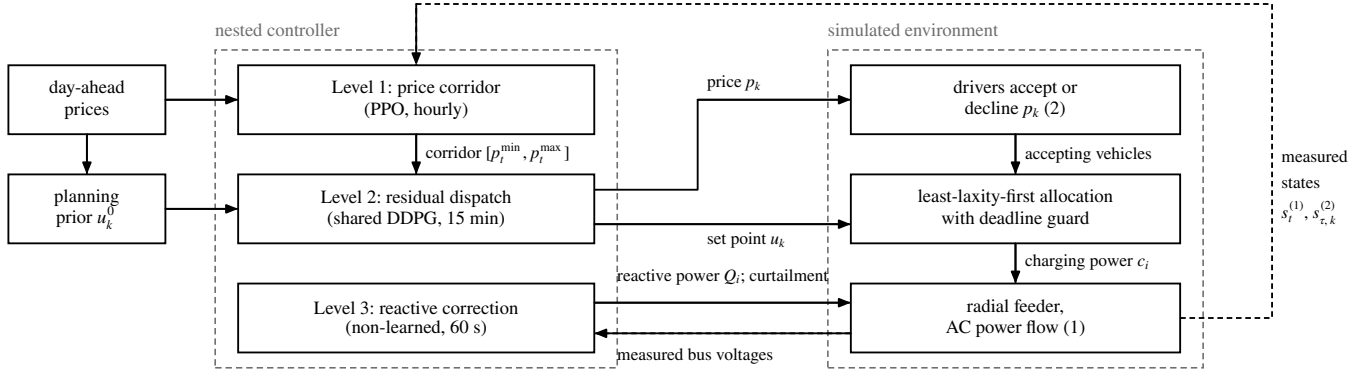
Fig. 2. Nested controller and simulated environment. Solid arrows are set points and data passed down; dashed arrows are measurements fed back. Labels name the quantity passed; numbers in parentheses refer to equations.
