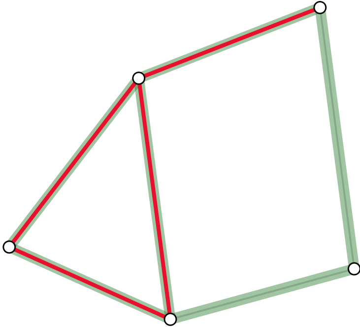
clean graph
