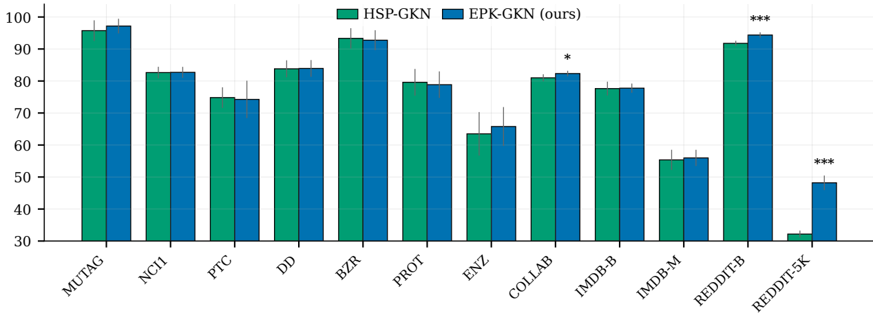
accuracy (%)
