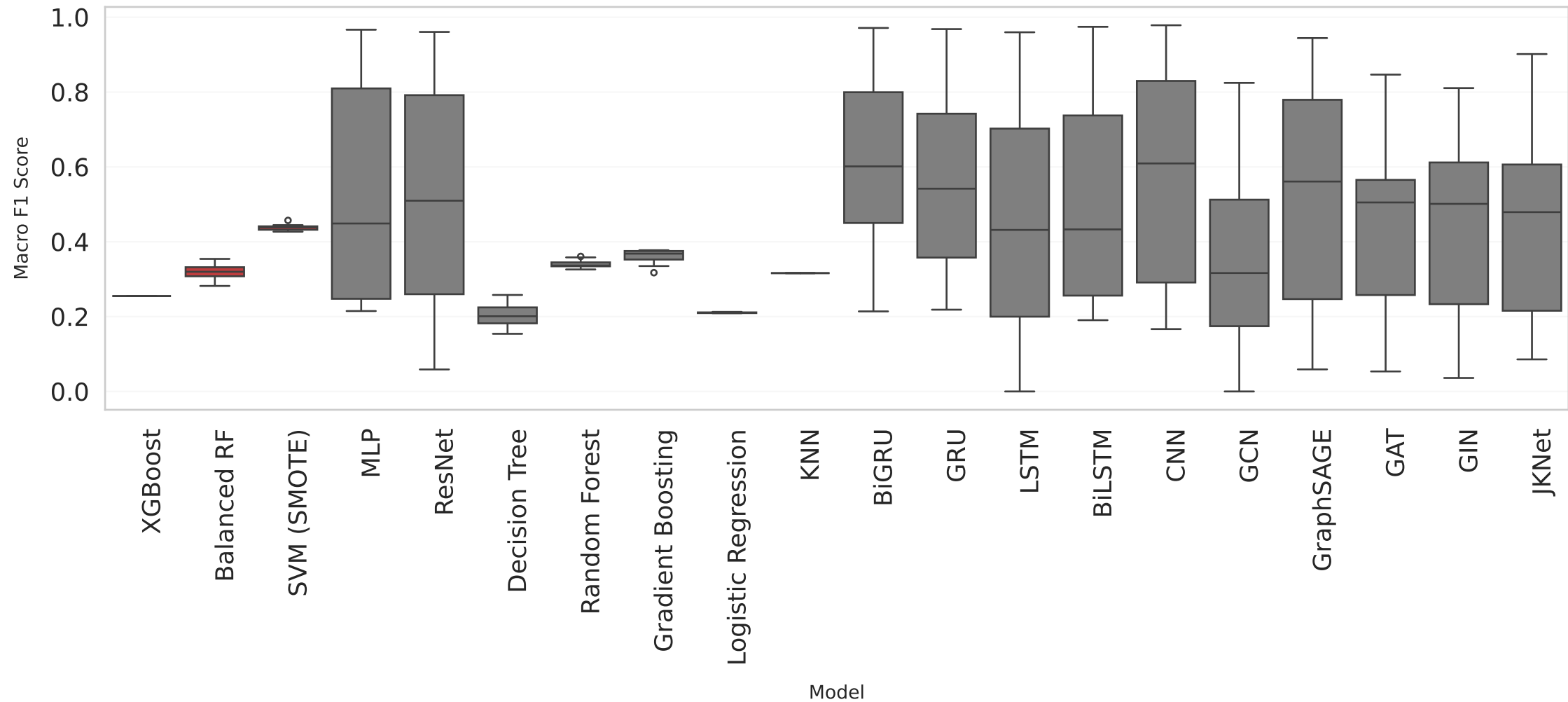
Cross-Dataset Performance Distribution
