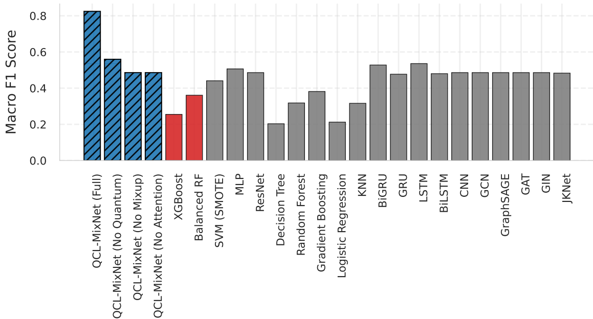
Performance on arrhythmia
