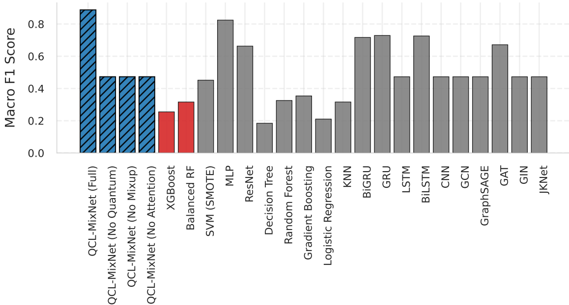
Performance on ecoli
