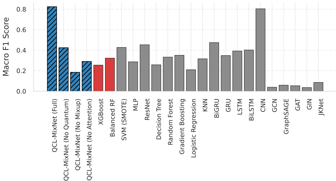
Performance on one-hundred-plants-texture
